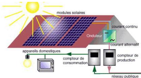
Installation photovoltaïque individuelle
